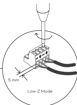
Output cable connections
