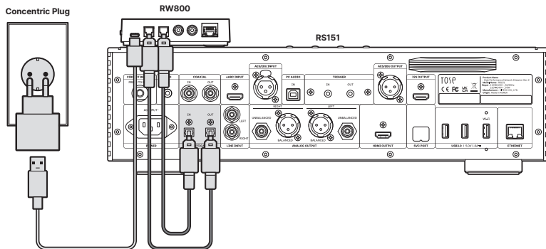
Concentric Plug
